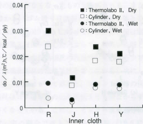
図6 Thermal resistance of different inner cloth
