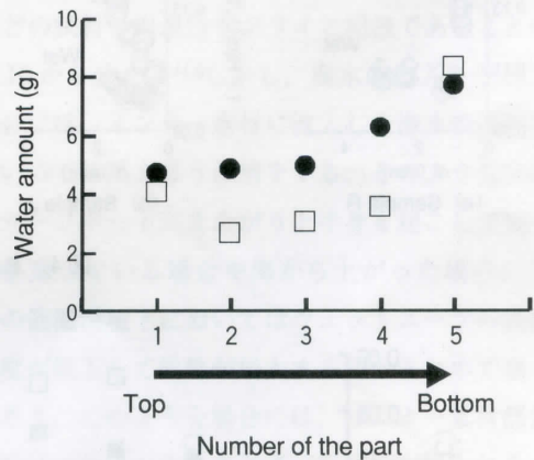
図7 Water distribution by using the cylinder method
