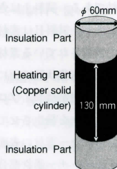
図1 Heated body
