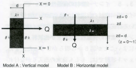
図8 Simple model based on water transfer
