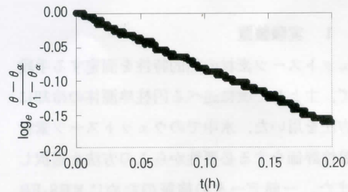
図3 Estimation of K value
